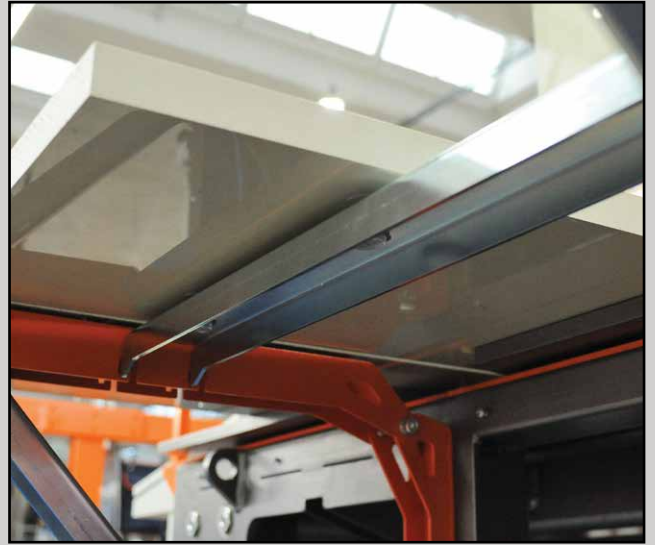
Connecting beams for lateral supports, allow positioning short sheets
